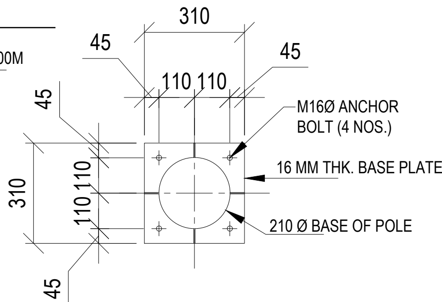
DETAIL OF BASE PLATE
