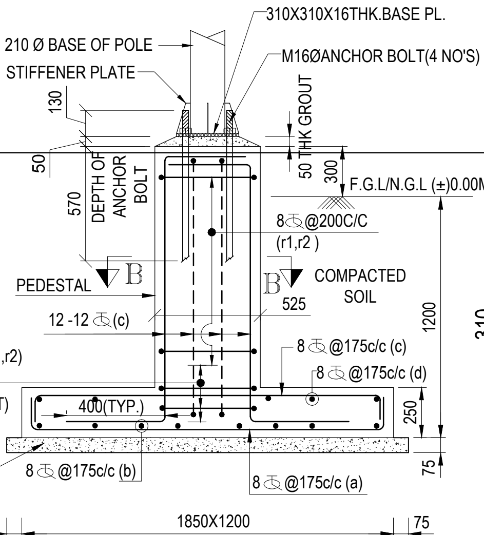
SECTION OF -A-A
