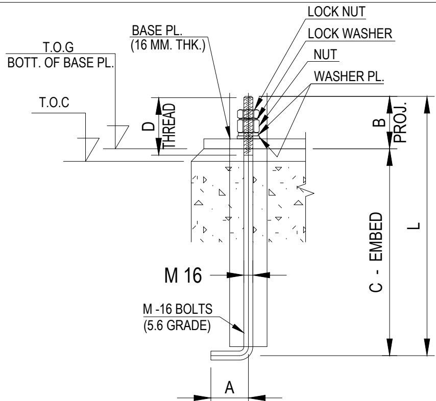
TYPICAL DETAIL OF ANCHOR BOLT
