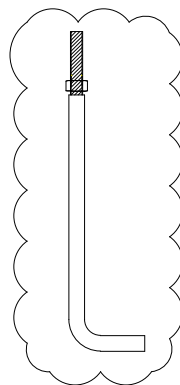
REFER FOUNDATION DRAWING FOR FOUNDATION BOLT
