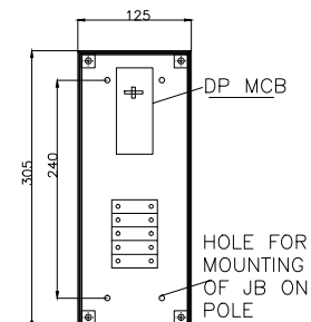
JB FRONT VIEW WITHOUT DOOR
