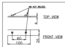
DETAIL B JB HOLDING STRIP
