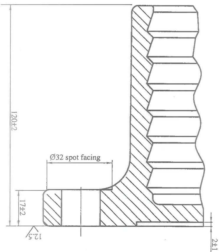
DETAILS AT 'A'
