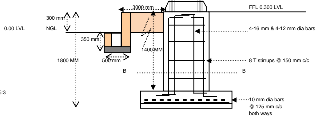
REINFORCEMENT DETAILS
