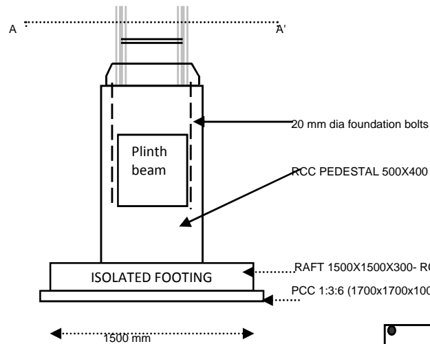
COLUMN FOOTING/PEDESTAL
