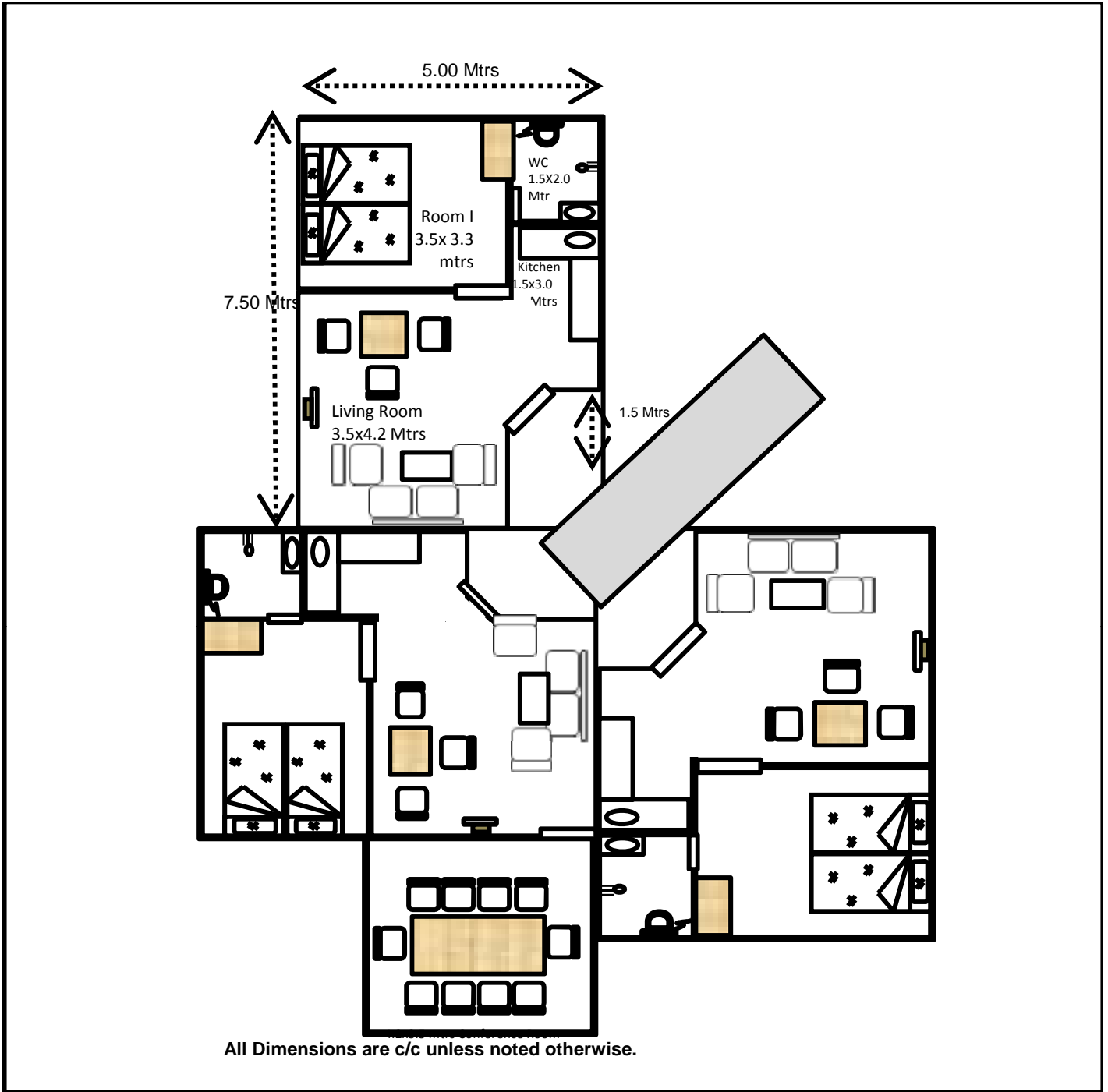
TYPICAL 'A' TYPE LIVING ACCOMODATION
