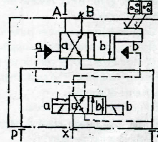
Fig-2 SYMBOL DIAGRAM
