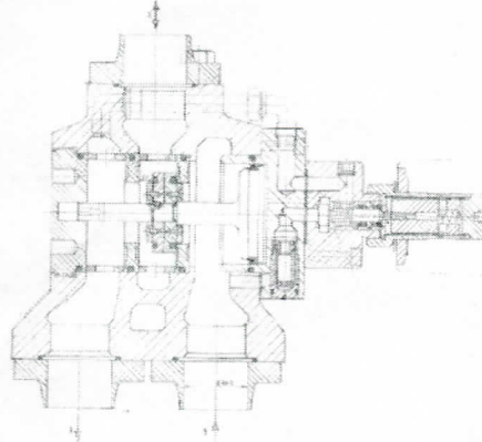
Fig-1 SCHEMATIC VIEW OF SOLENOID VALVE
