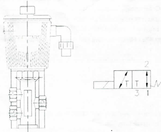
SCHEMATIC VIEW OF SOLENOID VALVE
