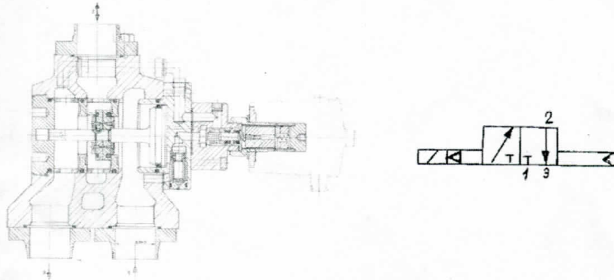
SCHEMATIC VIEW OF SOLENOID VALVE
