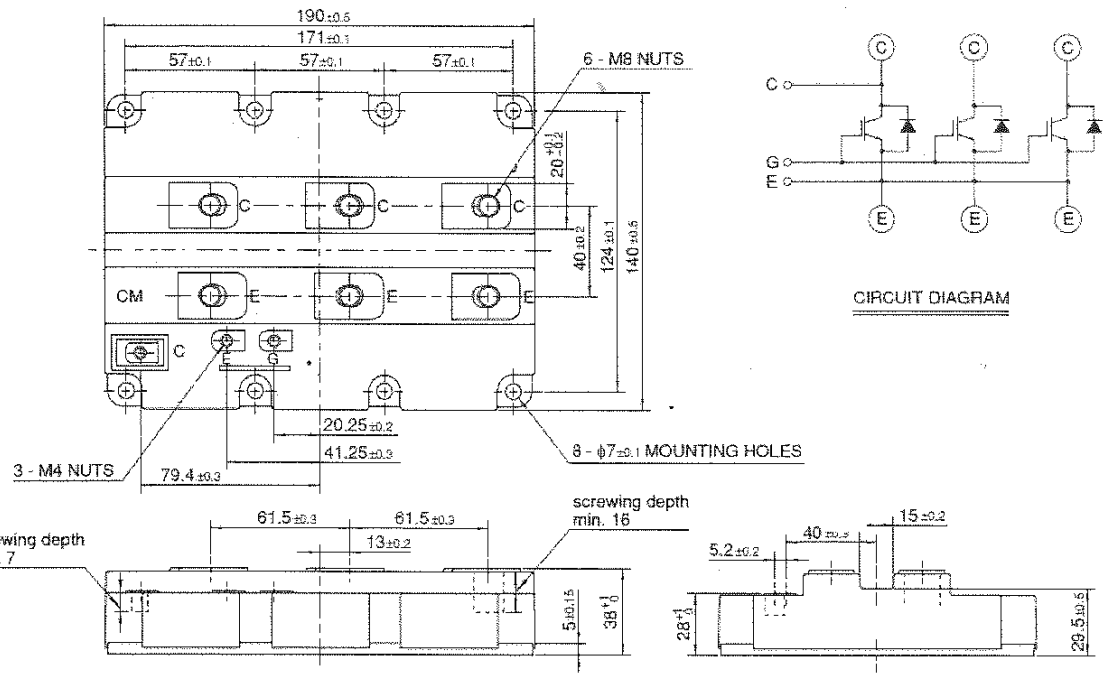
Outline drawing (for dimensional purpose only)
