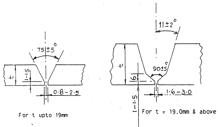
Fig.4: Plate Butt Weld Specimen
