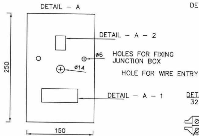
SMC JUNCTION BOX INSIDE VIEW
