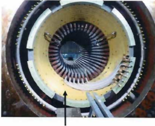
For support and consolidation of the overhang structure of large size TG (above 500 MW ratings).
