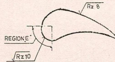
PROFILE SURFACE FINISH
