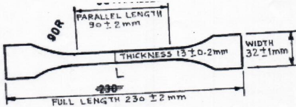
Fig. 1 Specimen for Tensile Strength Test.
