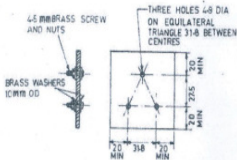
Fig. 12 Specimen And Electrodes
