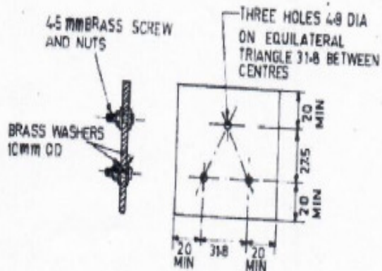
Fig. 12 Specimen And Electrodes
