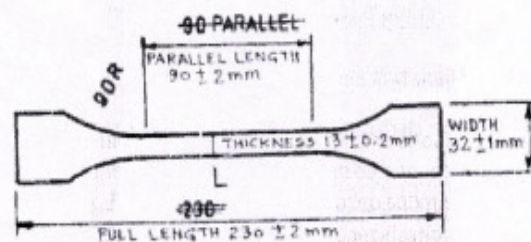
Fig. 1 Specimen for Tensile Strength Test.
