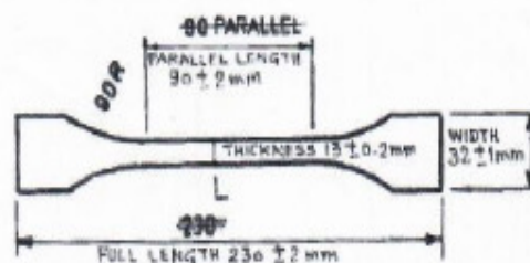
Fig. 1 Specimen for Tensile Strength Test.
