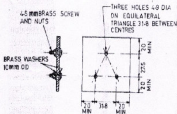
Fig. 12 Specimen And Electrodes
