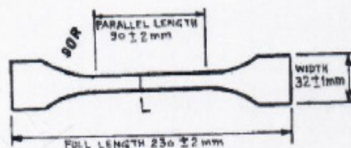
Fig. 1 Specimen for Tensile Strength Test.
