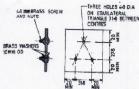
Fig. 12 Specimen And Electrodes
