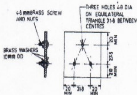
Fig. 12 Specimen And Electronics
