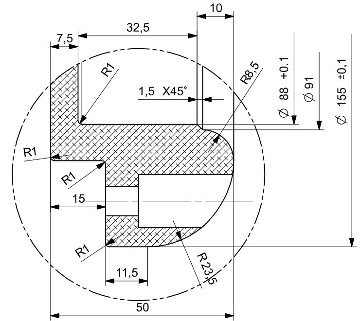
DETAIL C SCALE 3:2
