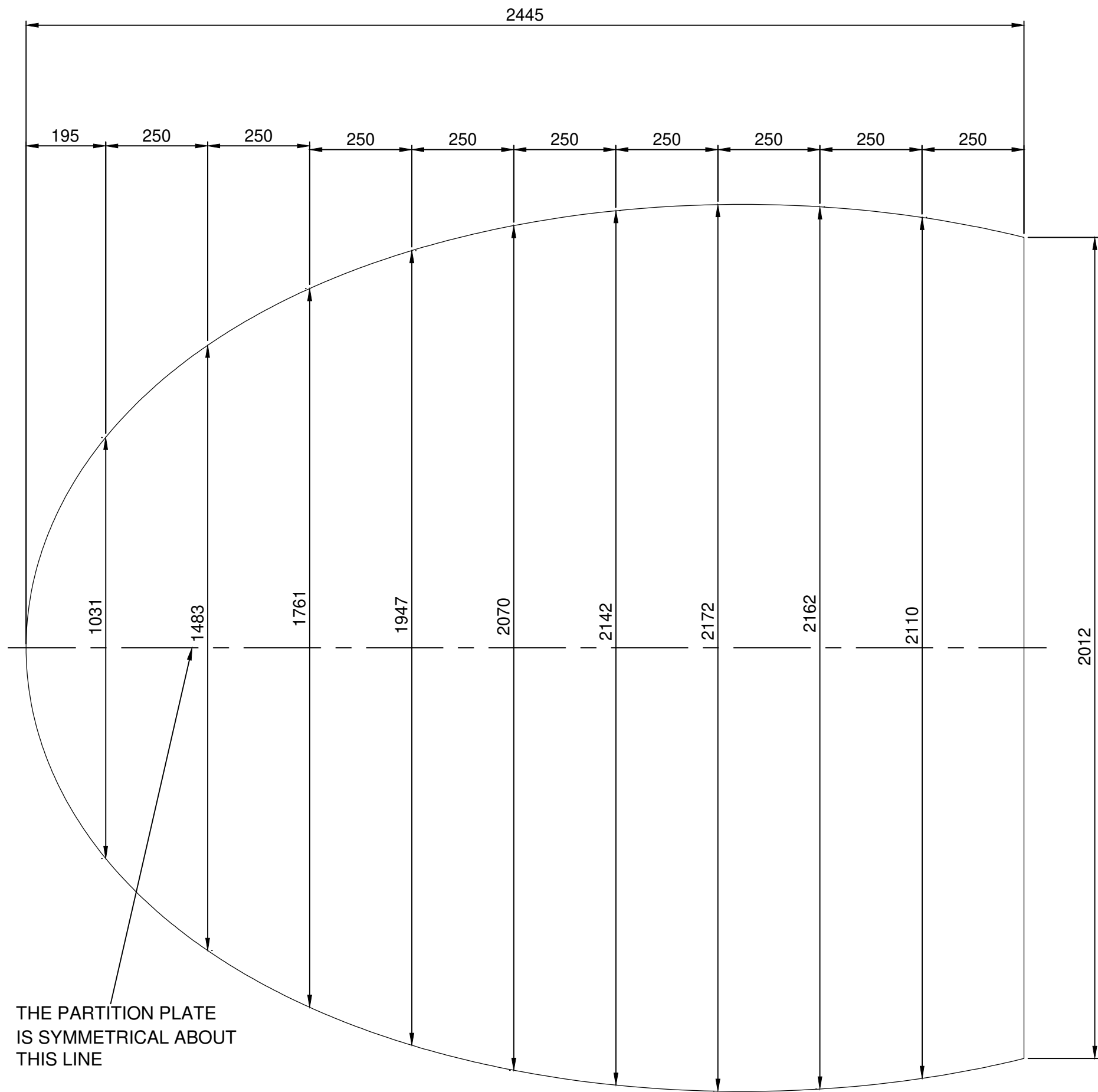
DEVELOPED VIEW
