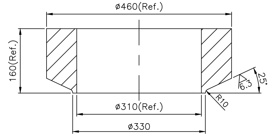
PRE-MACHINING DETAILS
