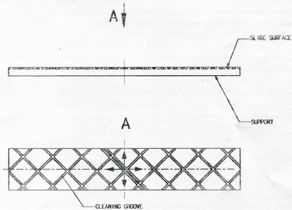
Schematic View of Lubricating Plates
