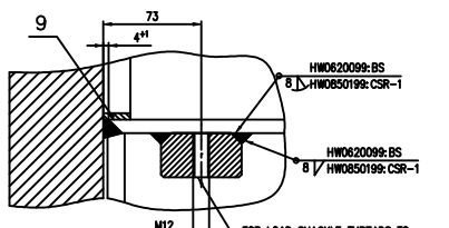
SECTION-DD SCALE:-1:2
