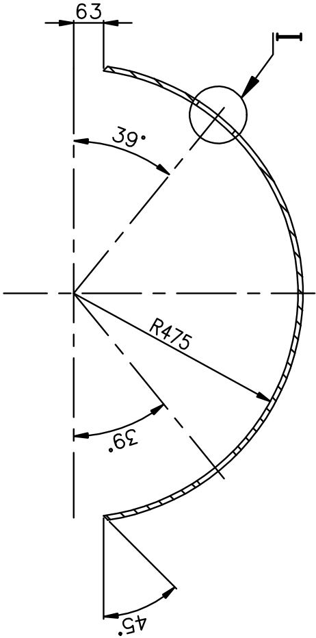
SECTION AA
