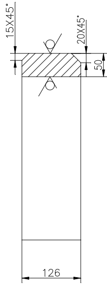
SECTION-AA
