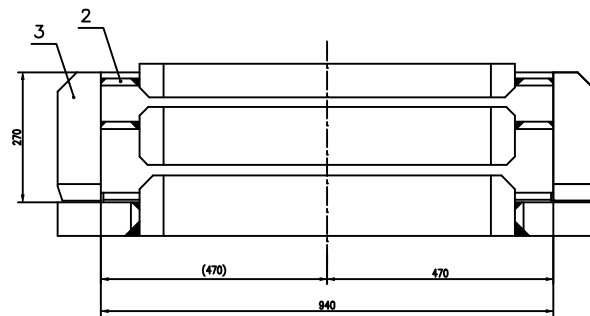
VIEW ON THE JOINT PLANE OF UPPER HALF
