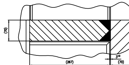
SECTION-CC SCALE:-1:2.5
