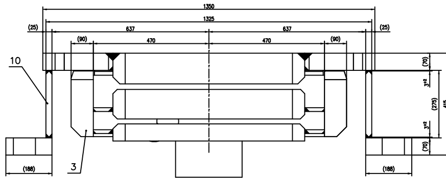
VIEW ON THE JOINT PLANE(UPPER PART)
