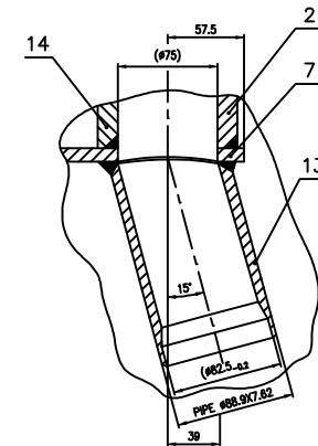
SECTION-BB SCALE:-1:2
