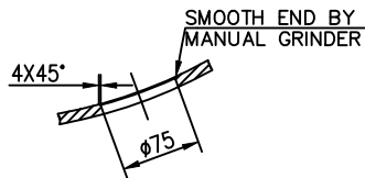
VIEW-Z SCALE-1:5
