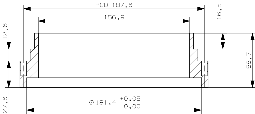
SECTION G-G
