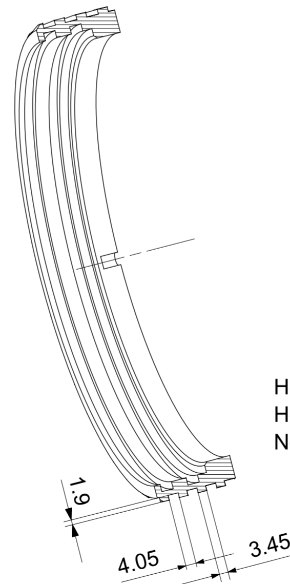
SECTION U-U
