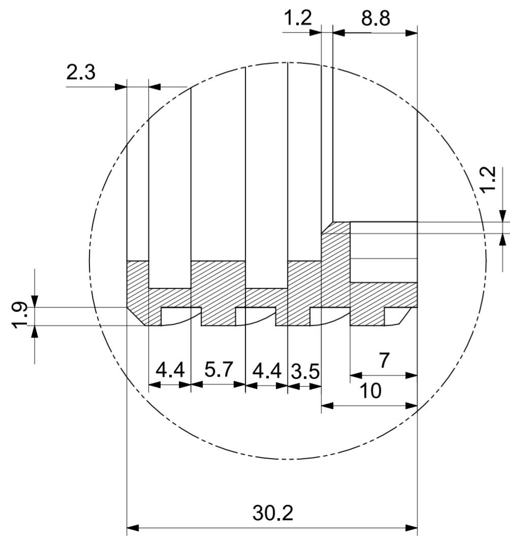
DETAIL T SCALE 5:2
