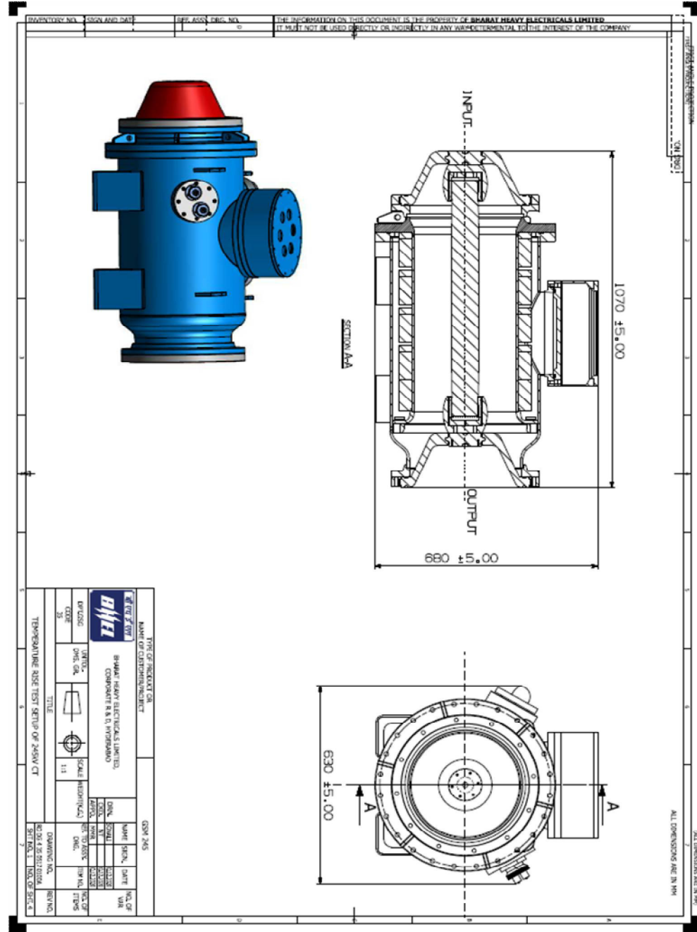
Figure 3 245kV Current Transformer module
