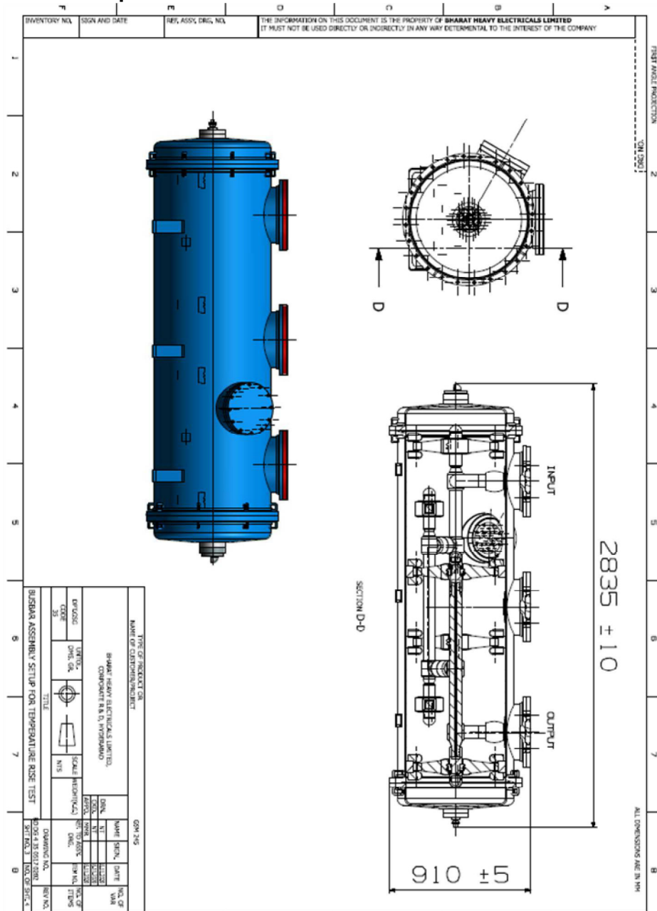
Figure 2 245kV Compact Bus duct Module
