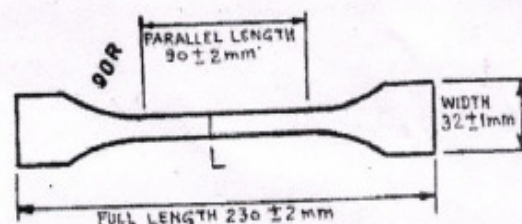
Fig. 1 Specimen for Tensile Strength Test.
