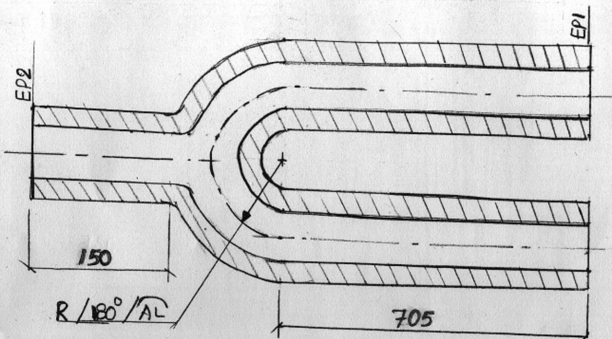
DETAILS OF 500 MW BIFURCATES – SKETCH-B
