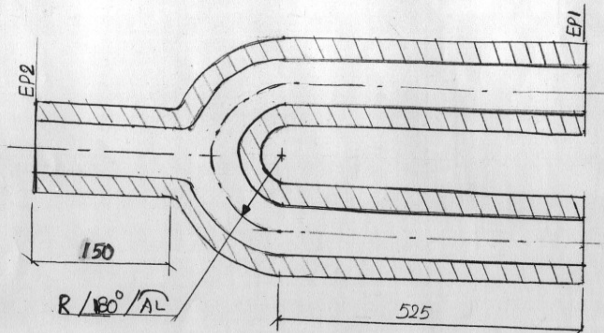
DETAILS OF 500 MW BIFURCATES – SKETCH-A
