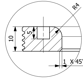
DETAIL C SCALE 2:1
