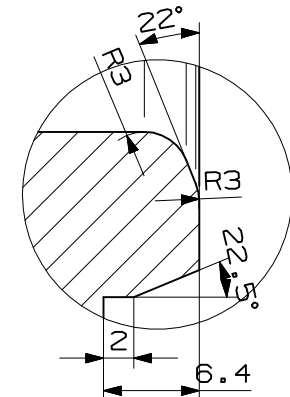
DETAIL B SCALE 3:1
