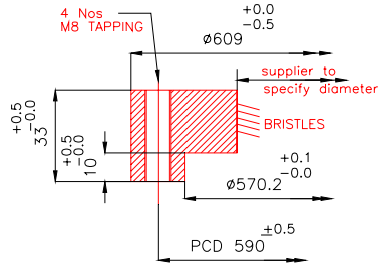
BRUSH SEAL WITH MOUNTING RING (Single piece design)
