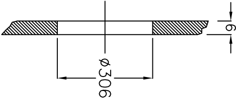
Detail—A
