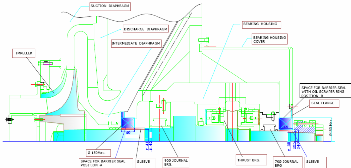
FIG.1. BARRIER SEAL ARRANGEMENT IN HIGH SPEED COMPRESSOR TEST RIG
