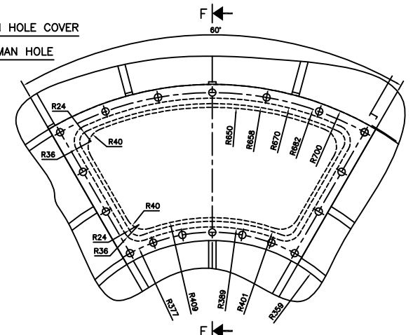
MAN HOLE ASSEMBLY DETAIL-X
