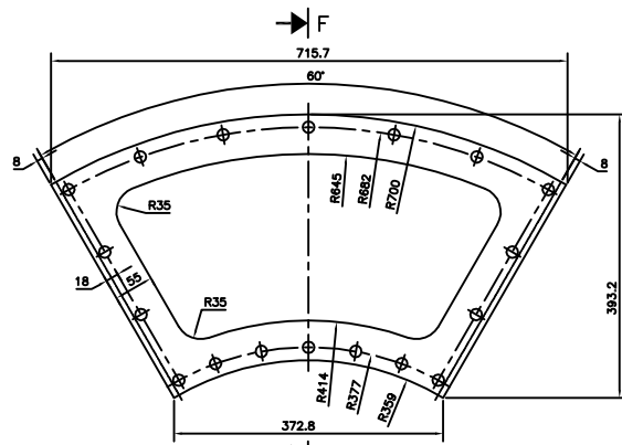
MAN HOLE COVER
