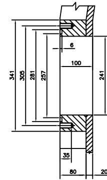
SECTION G-G
