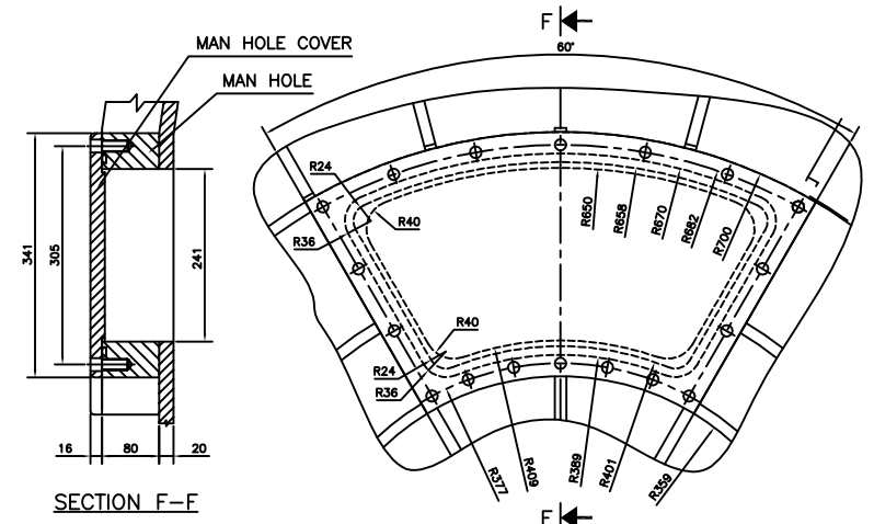
MAN HOLE ASSEMBLY DETAIL-X
