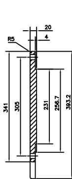
SECTION F-F
