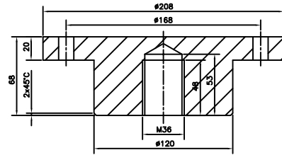
SENSOR HOLDING COVER
