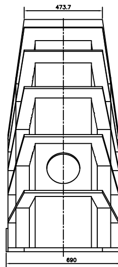
SIDE VIEW C-C
