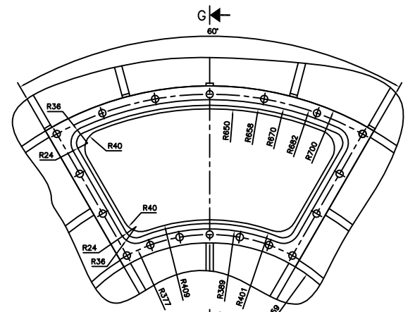
MAN HOLE DETAIL-X
