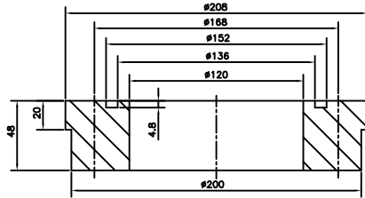
SENSOR SUPPORT BRACKET
