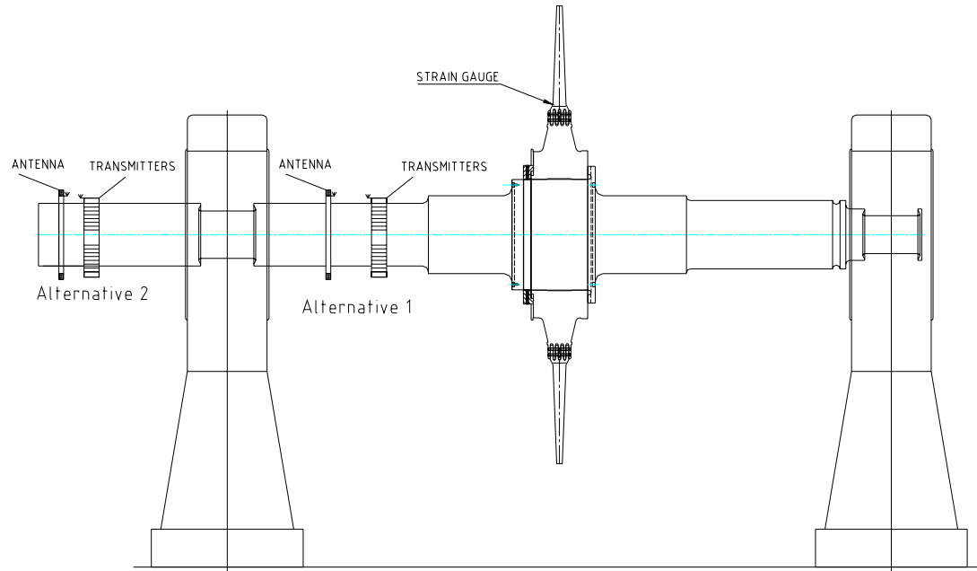
SCHEMATIC FOR TELEMETRY INSTRUMENTATION
