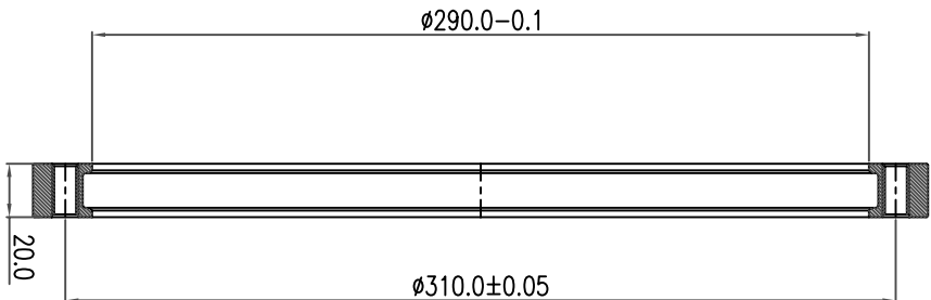
SECTION AA
