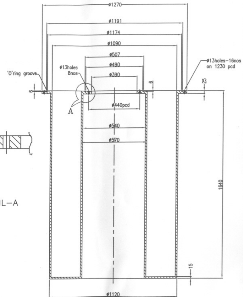
INNER CONTAINER Material: FRP
