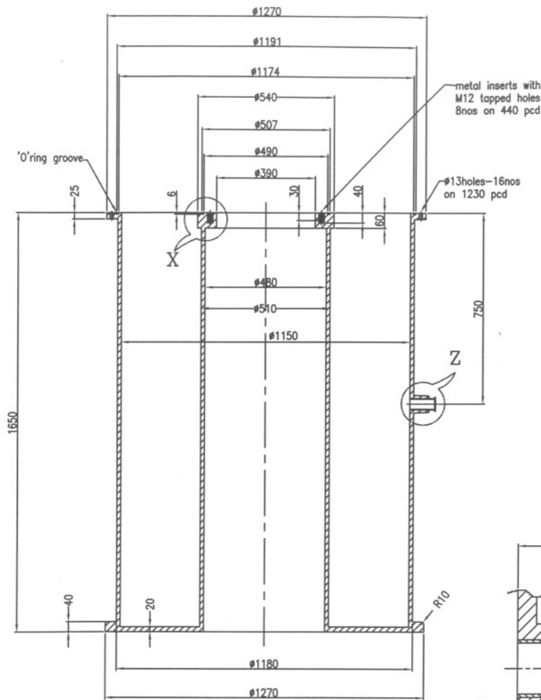
OUTER CONTAINER Material: FRP
