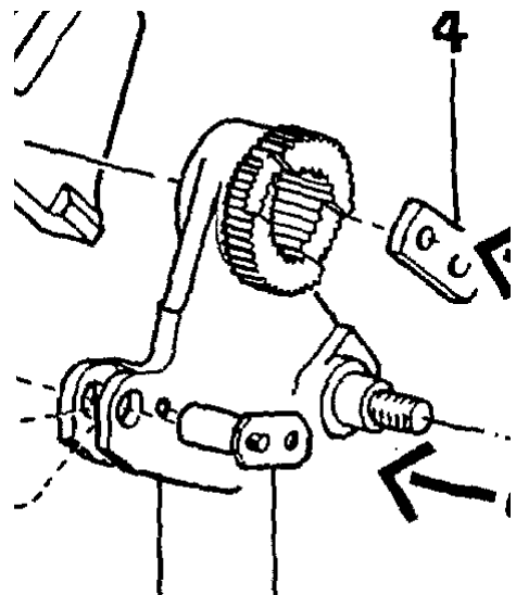
CRANK OUTER
