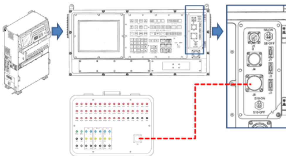
Connection Diagram
