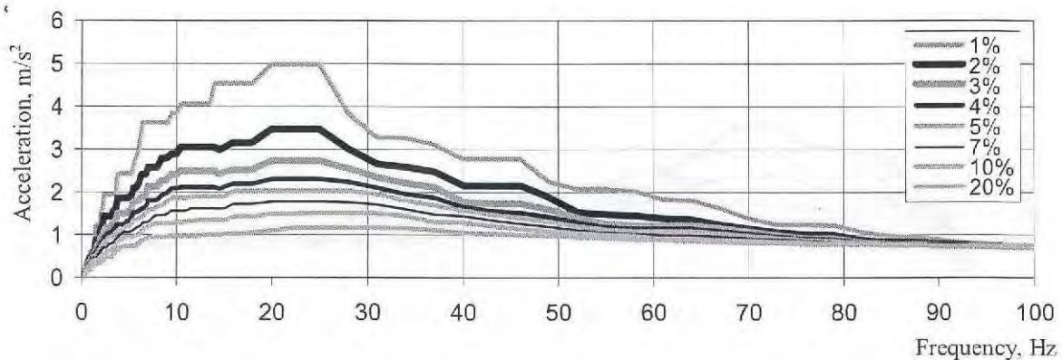
a) Along the horizontal grid x ( \text{ZPA} = 0.77 \text{ m/s}^2 )
