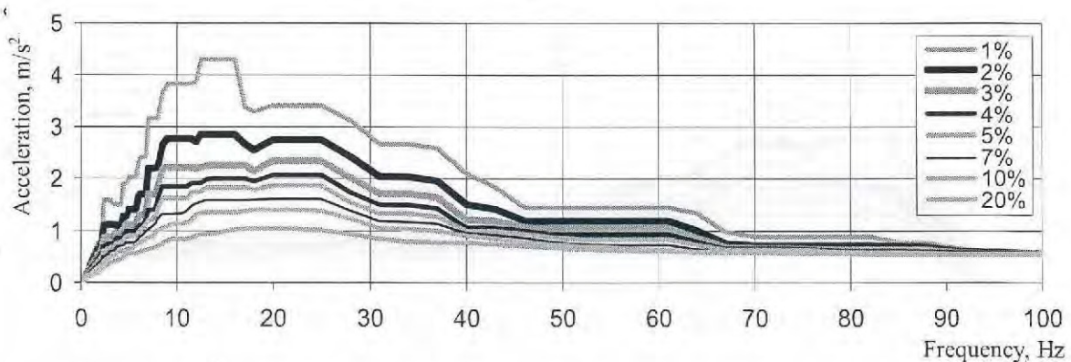
b) Along the horizontal grid y ( \text{ZPA} = 0.72 \text{ m/s}^2 )
