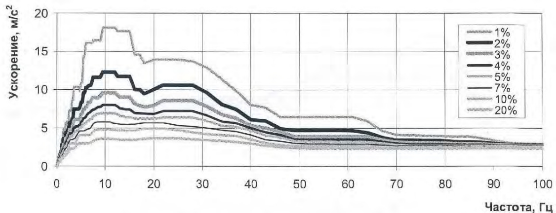
a) along the horizontal grid x (ZPA = 2,15 m/s 2 )
