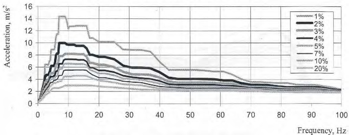
c) along the vertical grid z (ZPA = 1,86 m/s 2 )
