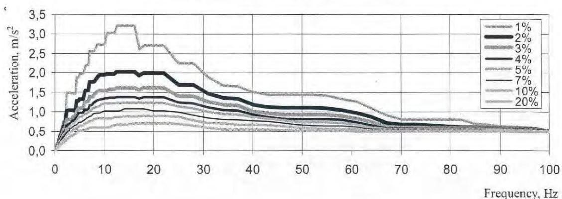
c) Along the vertical grid z ( ZPA = 0.47 m/s^2 )
