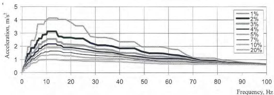
a) Along the horizontal grid x ( ZPA = 0.54 m/s^2 )
