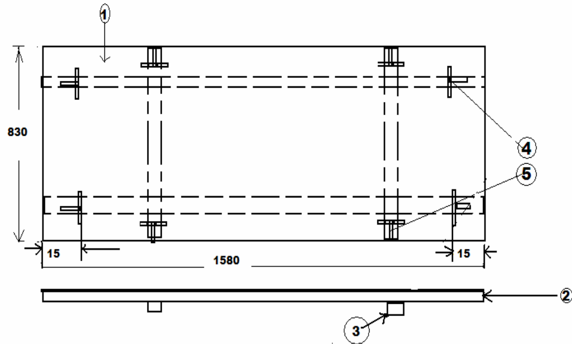
Base Plate of Box for Operator Panel of Induction Heating Equipment
