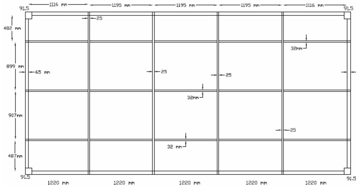
Plan of MS Top frame (size 20' x 10' x 8.5')
