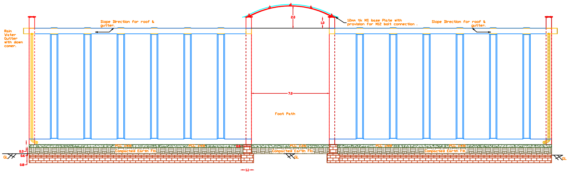
Front Elevation
