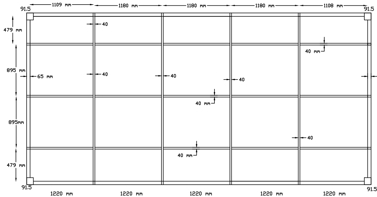
Plan of MS Base frame (size 20' x 10' x 8.5')
