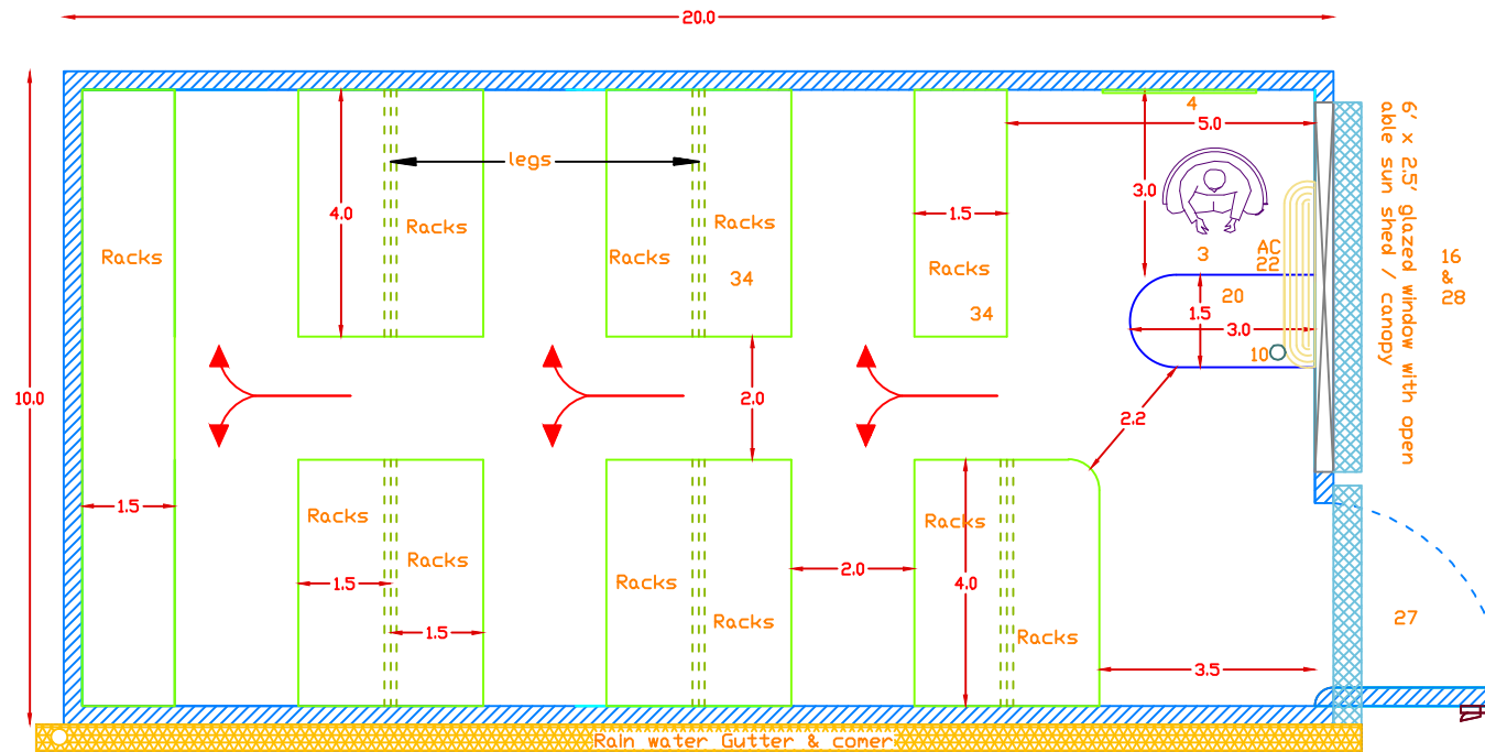
DOCUMENTATION ROOM - 20' X 10' - TYPE BUNK HOUSE.
