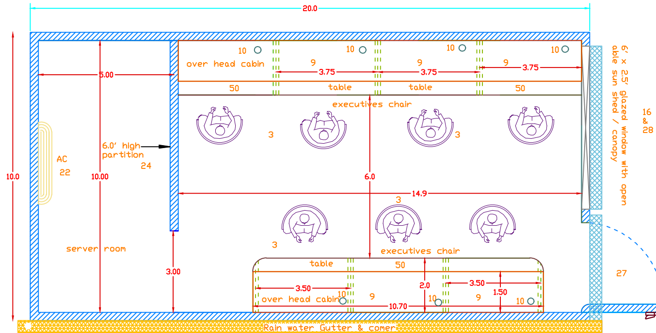
COMPUTER / SERVER ROOM - 20' X 10' - F TYPE BUNK HOUSE.
