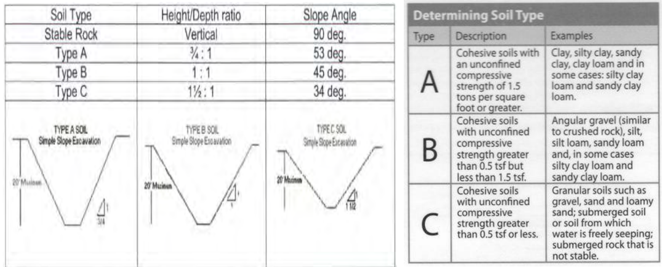
Fig. 13.2.2.1 Excavation Reference
