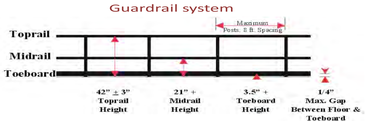
Fig. 13.2.1.2 Guard Rail System
