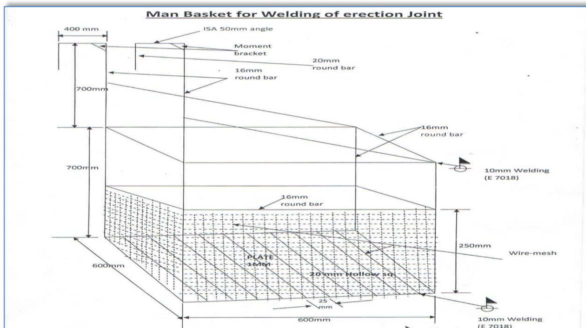
Fig. 5.1 Man Basket for Welding Erection Joint
