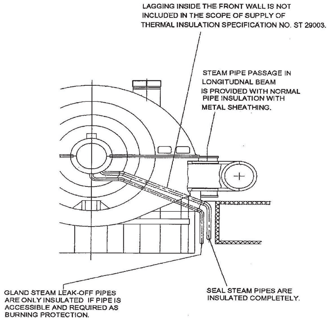
FIG.- 8 : L.P. TURBINE CASING.
