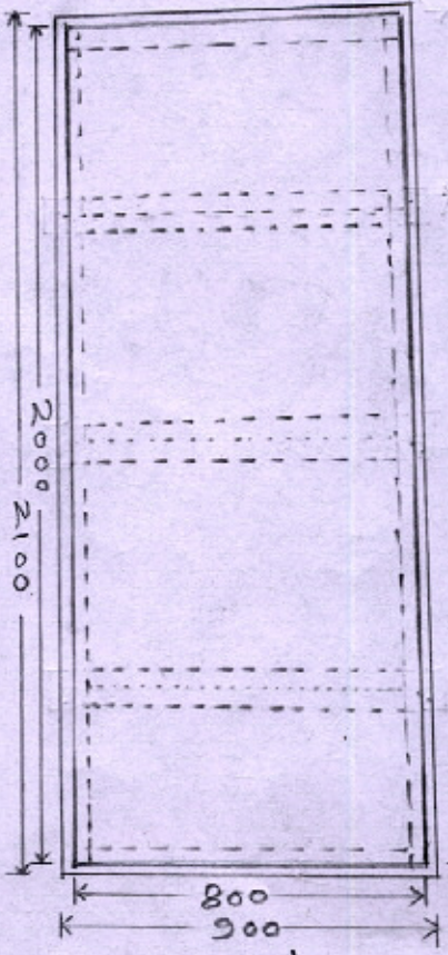
TOP VIEW
