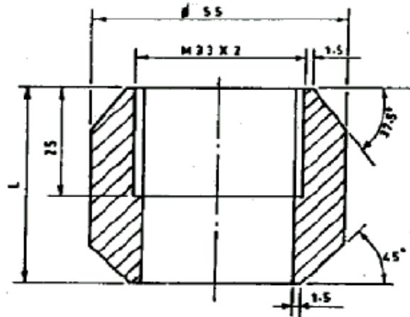
Figure-1: Stub Straight Immersion
