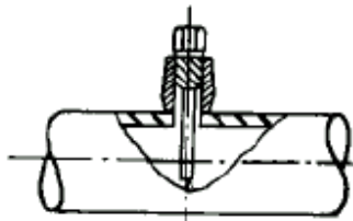
Figure-2: Straight Stub Installation on Pipe OD 168.3 and above
