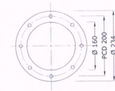
DETAIL VIEW - B X B DETAIL OF INLET & COUNTER FLANGE
