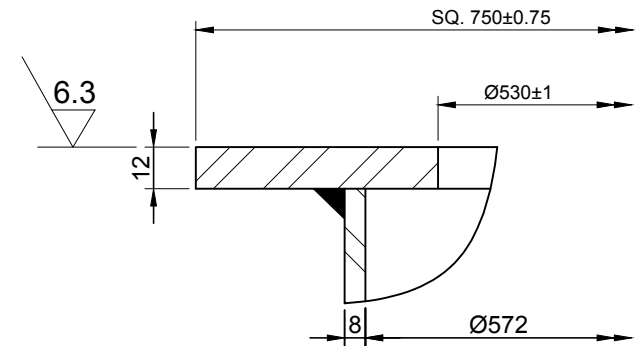
DETAIL - B
