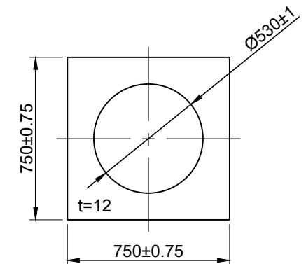
VIEW - X
