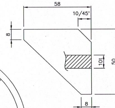
DETAIL-03
