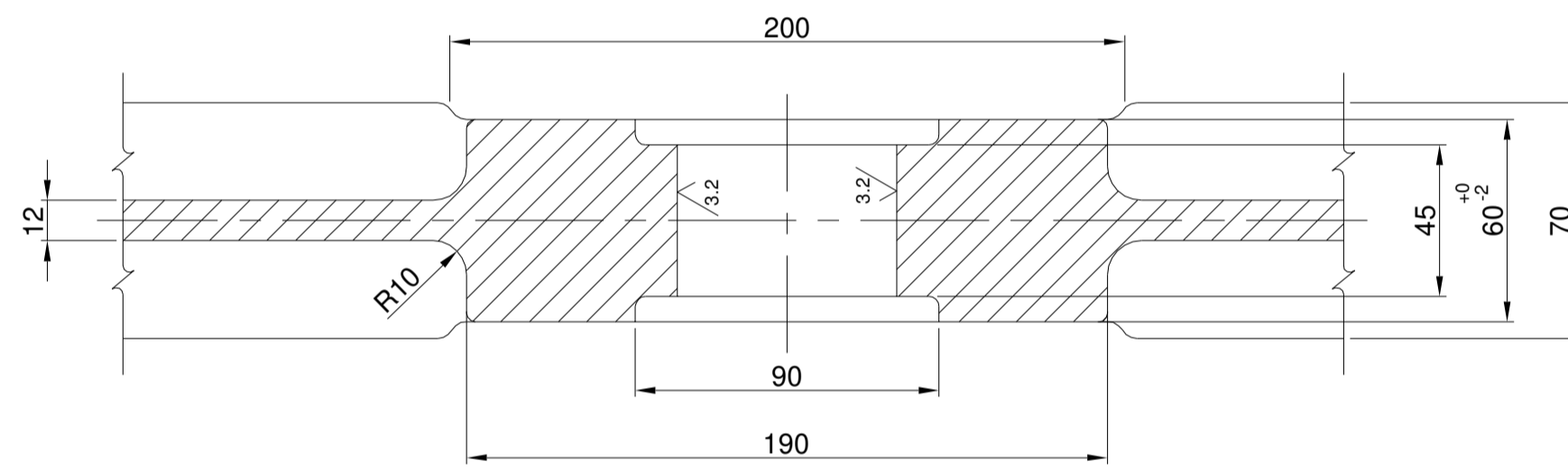
SECTION-BB
