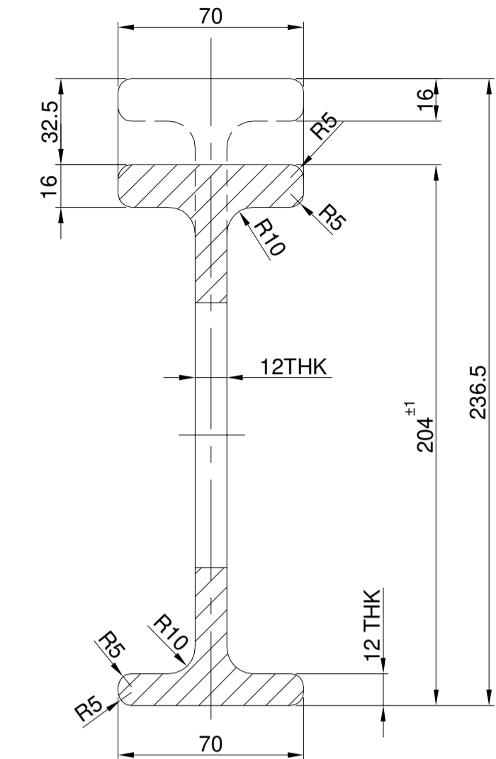
SECTION-CC
