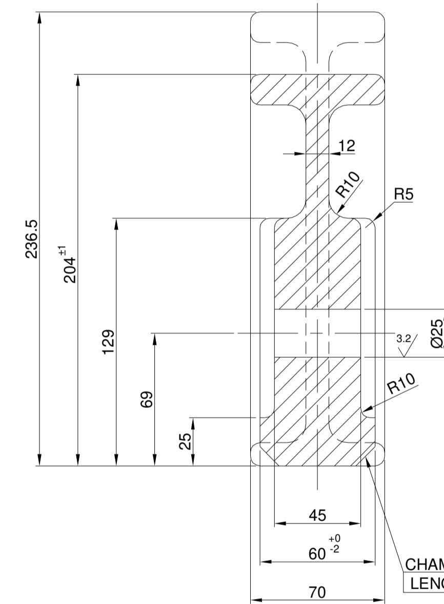
SECTION-DD
