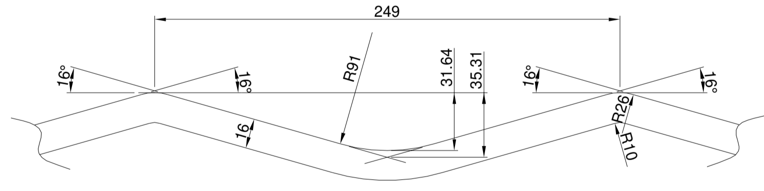
DETAIL-Y
