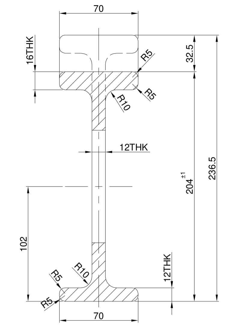
SECTION-CC
