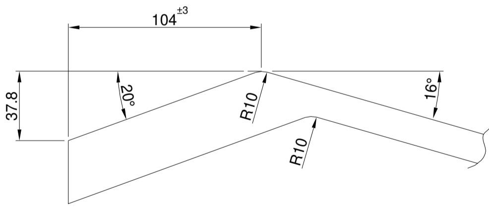
DETAIL-X
