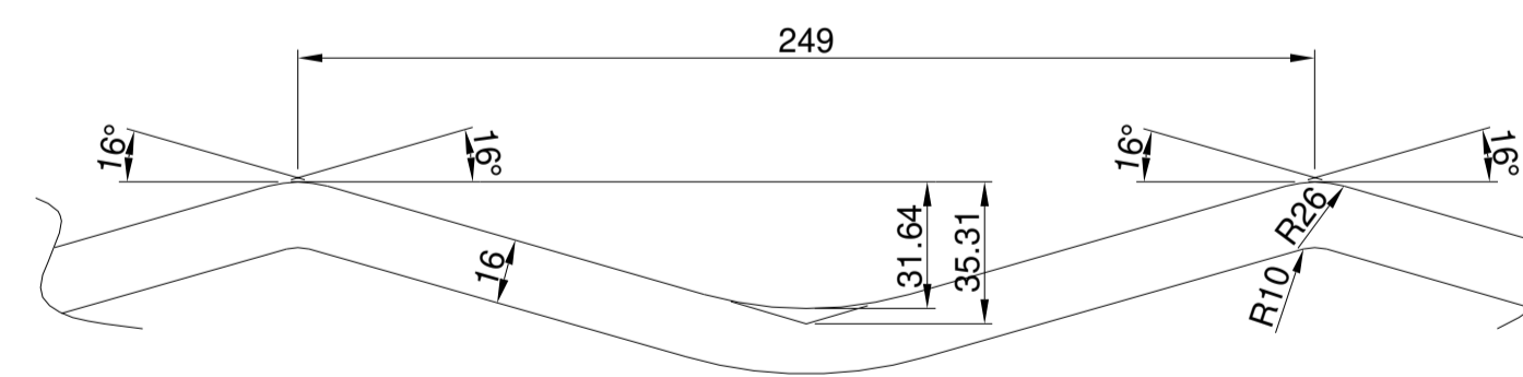
DETAIL-Y
