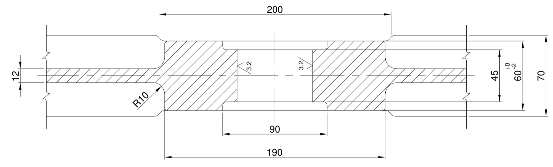
SECTION-BB
