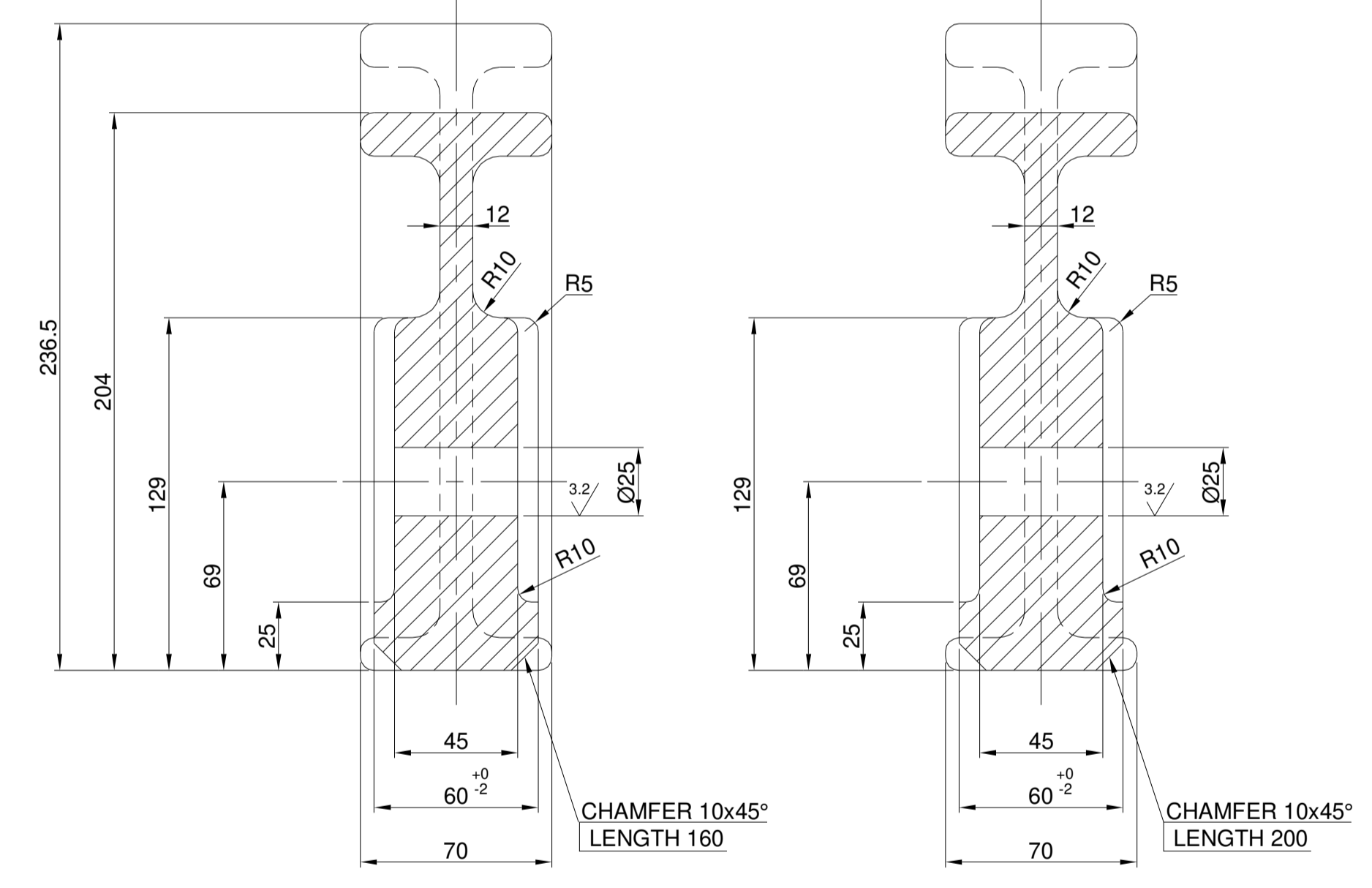
SECTION-DD
