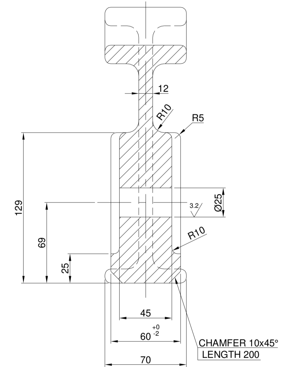
SECTION-EE
