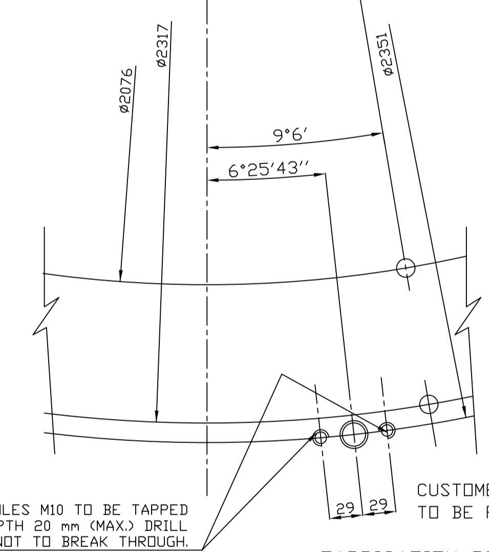
FABRICATION DRG. No.1-61-376-01307
