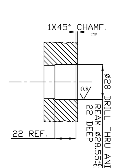
SECTION-DD
