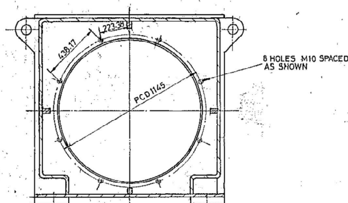
SECTION B-B (SEE NOTE)
